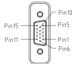
VGA FEMALE
